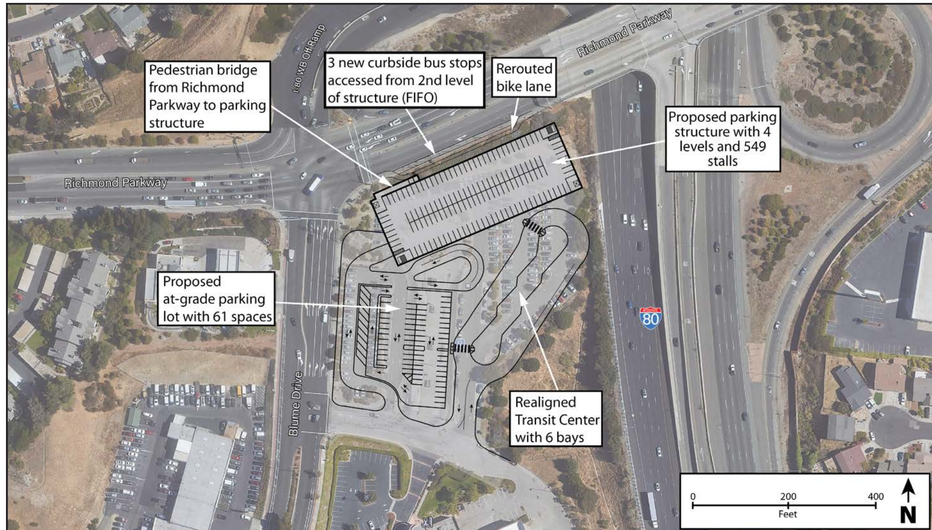
Figure 6-14 - Proposed Richmond Parkway Transit Center Capacity Enhancement (TC2)
