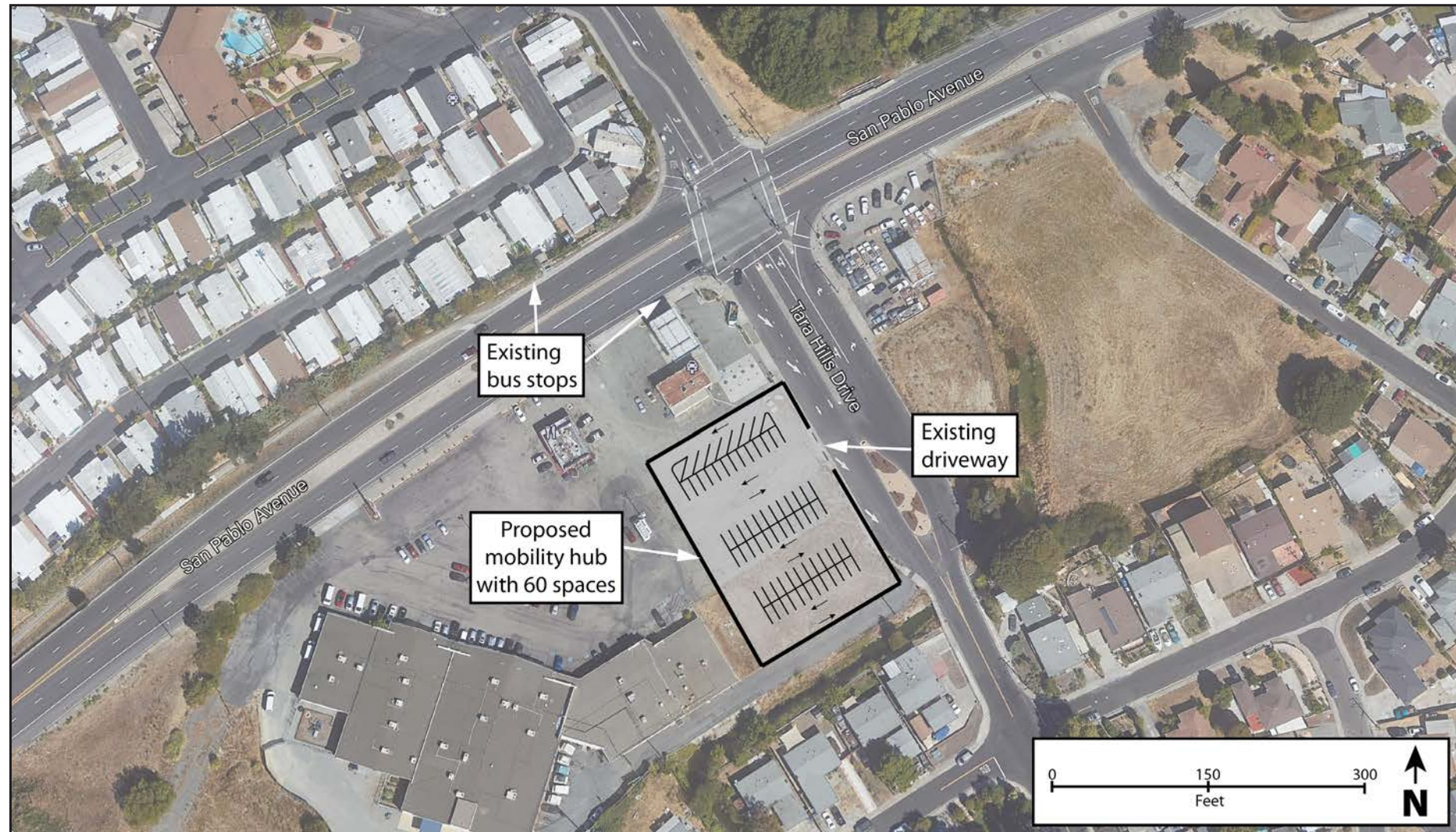
Figure 6-8 - Proposed Tara Hills Drive Mobility Hub, Option 1 (MH1)
