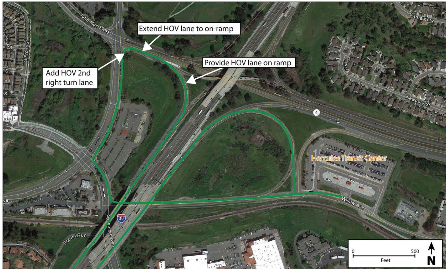
Figure 6-3 - SR-4/John Muir Parkway/I-80 Access Improvements (FA1)
